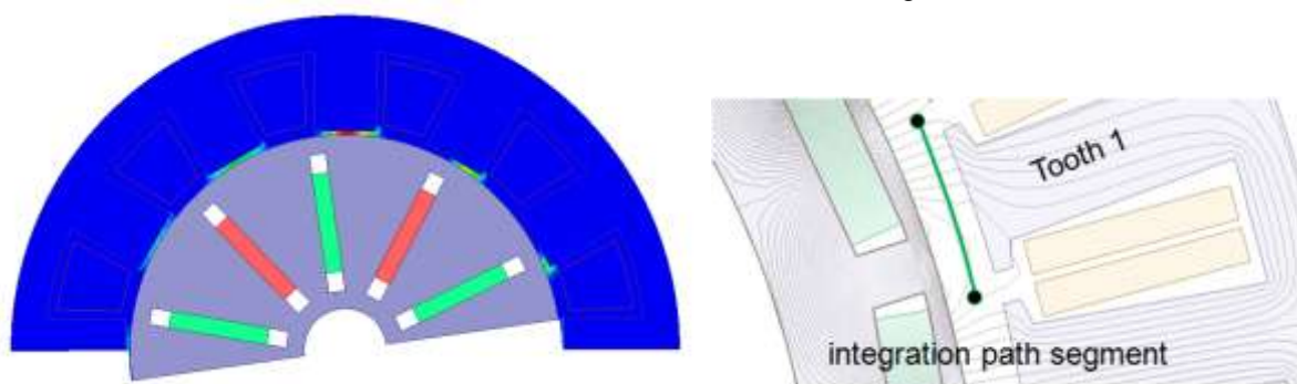
Fig. 3: Co-energy distribution inside the air gap and stator of a synchronous machine with permanent magnets and reduced force integration path
