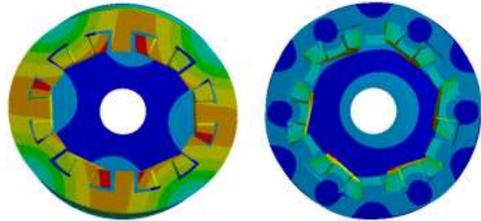
Fig. 2: Normal modes of outer parts of a motor
