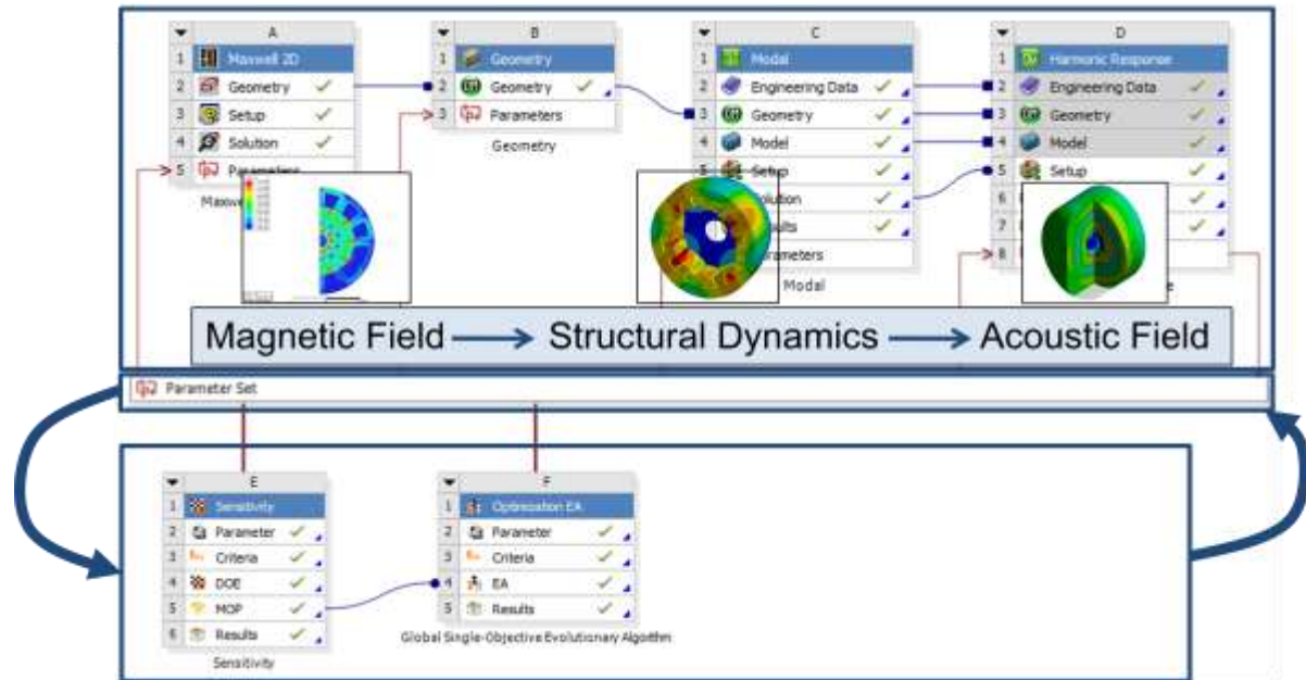
Fig. 4: Full parameterized optimization environment in ANSYS Workbench
