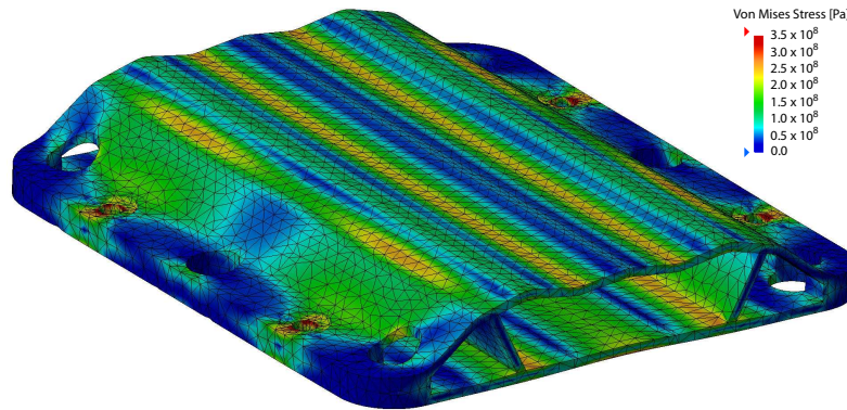
Figure 25: Von-Mises stresses of best plate design ever found. The plot also shows true scale deformations of the loaded structure.
