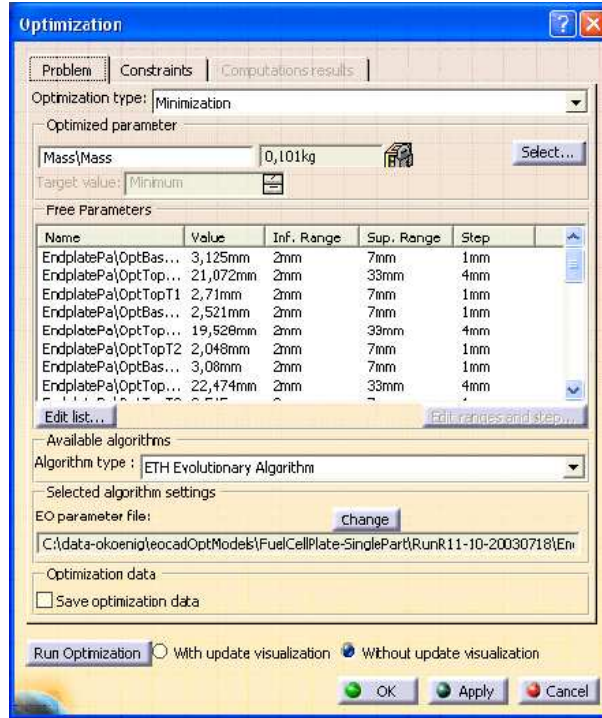
Figure 16: Integration of the generic EA into CATIA's optimization workbench.
