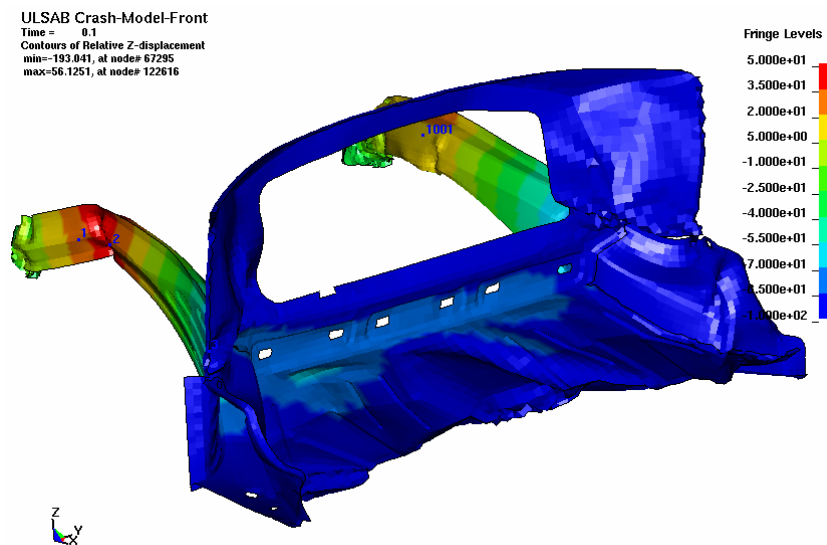
Figure 19: Design with Maximal Front Wall Intrusion
