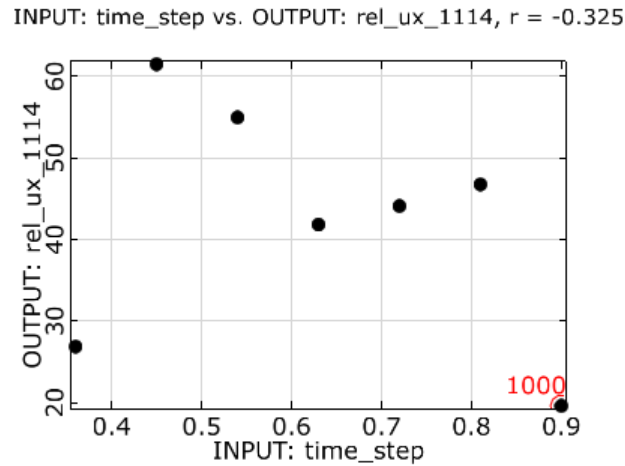
Figure 23: Anthill Plot of the Variation of the Critical Time Step Scaling concerning the Displacement of the Node 1114
