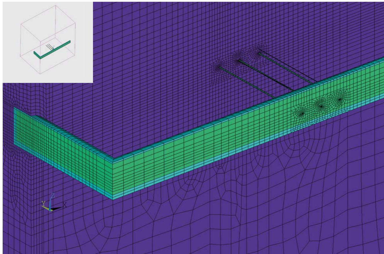
Figure 1: FE-mesh of structure, section
