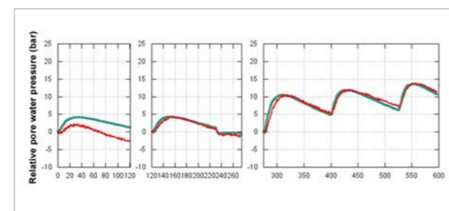
Figure 8b: Comparison of simulation vs. measurement at point 1252 after the parameter identification: Relative pore water pressure of the three heating periods
