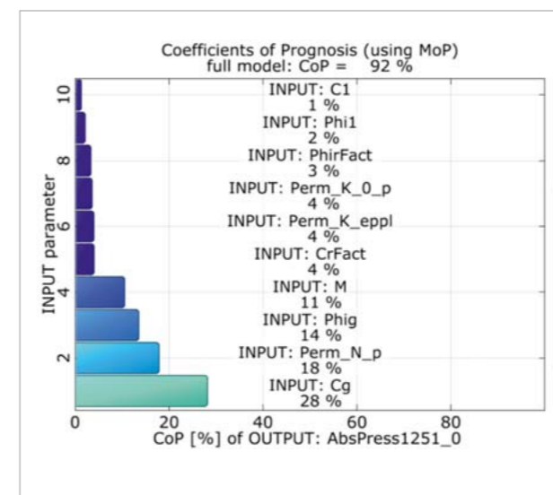
Figure 4: CoP relative pore pressure at time t = 0 , the measuring point in 1251
