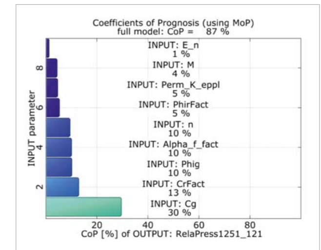
Figure 6: CoP relative pore pressure at time t = 121 days, measurement point 1251
