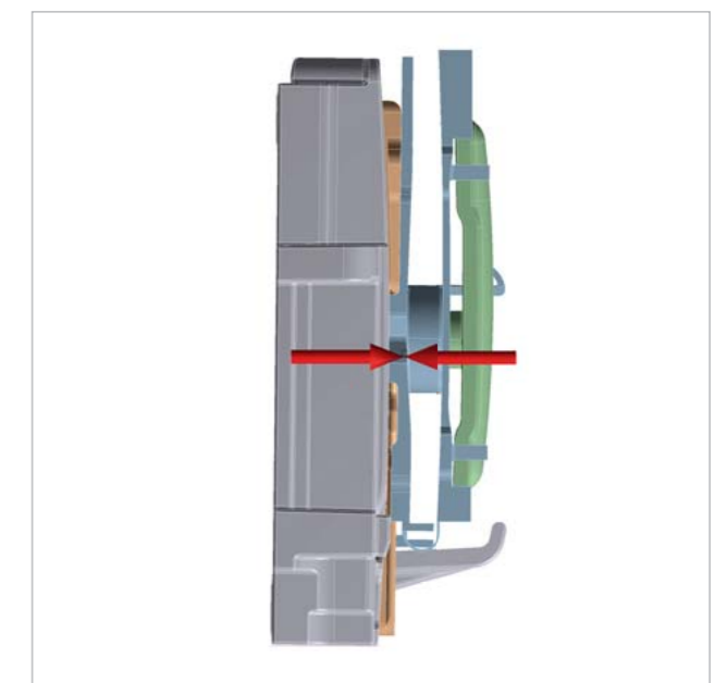
Clamp plate and rail slider assembly applies stress to glass. The arrows represent the bolt
